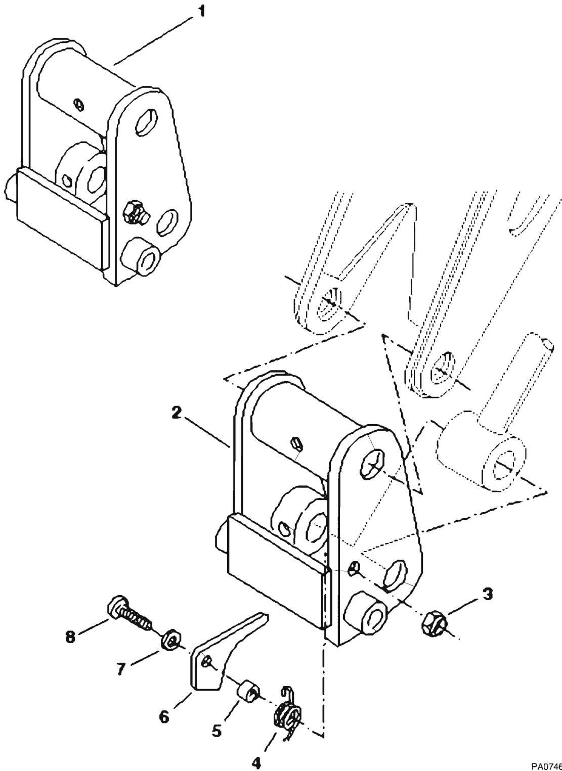
FIGURE 9-4. QUICK ATTACH
