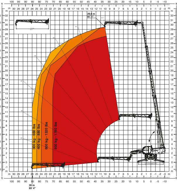
JW 800 Jib winch 800
