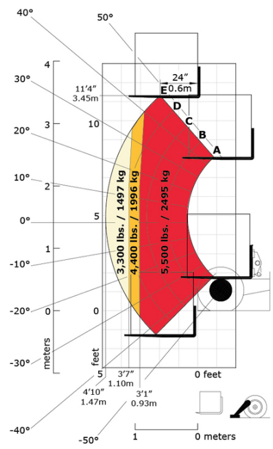
Machine on stabilisers with forks Imperial
