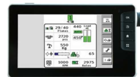
Automatic density control through the FieldStar 5 baler terminal.
